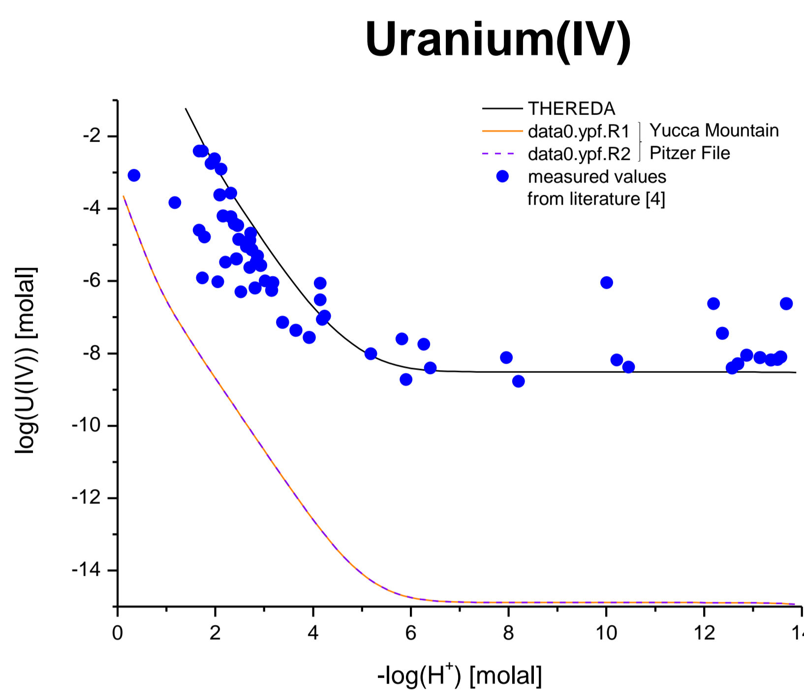
Fig. 1: Solubility of U(OH) 4 (am) in 1 m NaCl solution at T = 25 °C.
