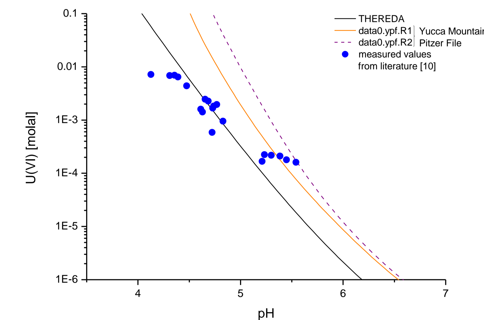
Fig. 5: Solubility of Becquerelite in 1 m CaCl 2 solution at T = 25 °C.
