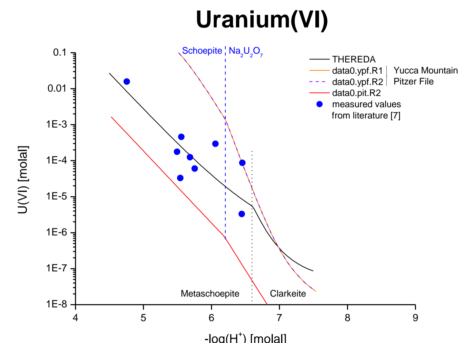
Fig. 4: Solubility of Metaschoepite in 5 m NaCl solution at T = 25 °C.
