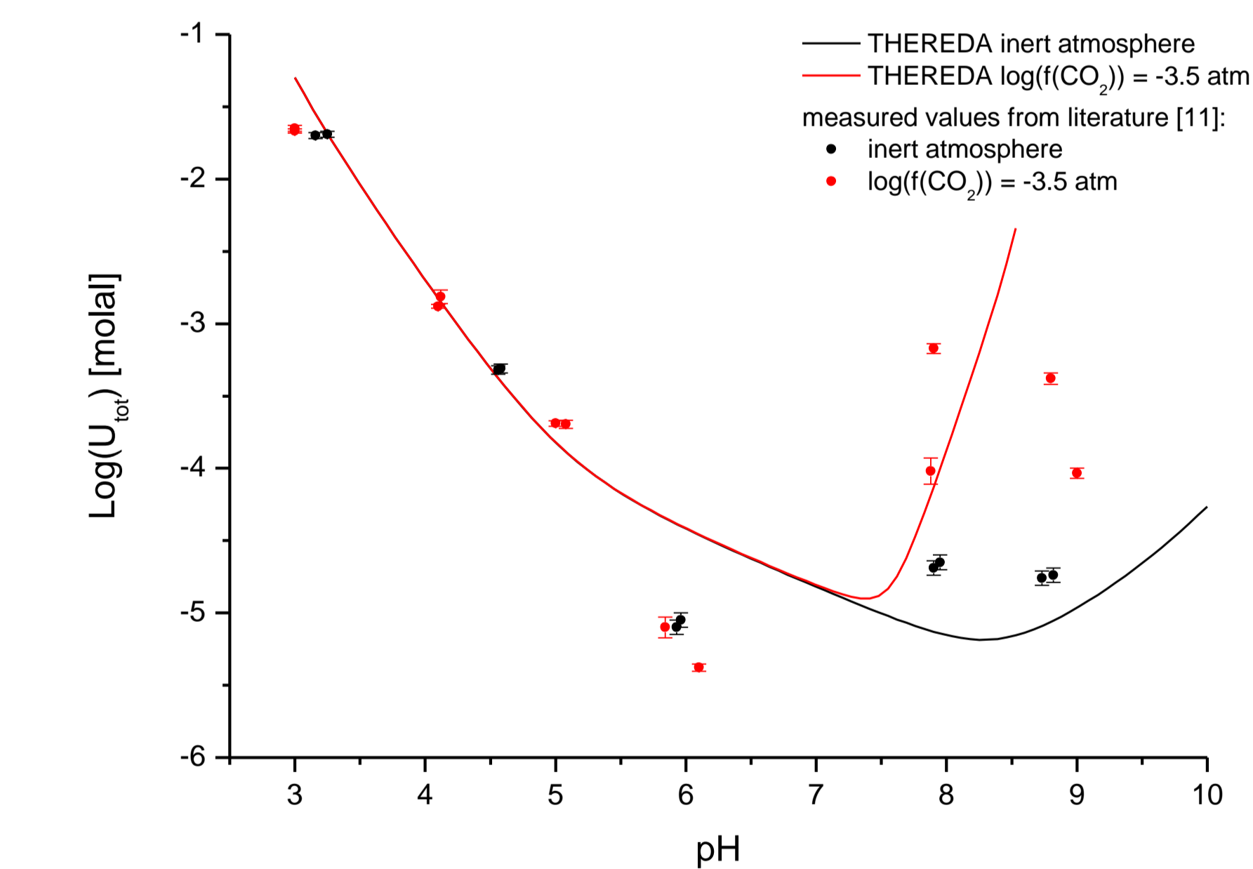
Fig. 6: Solubility of Soddyite in 0.1 M NaClO 4 solution at T = 25 °C.
