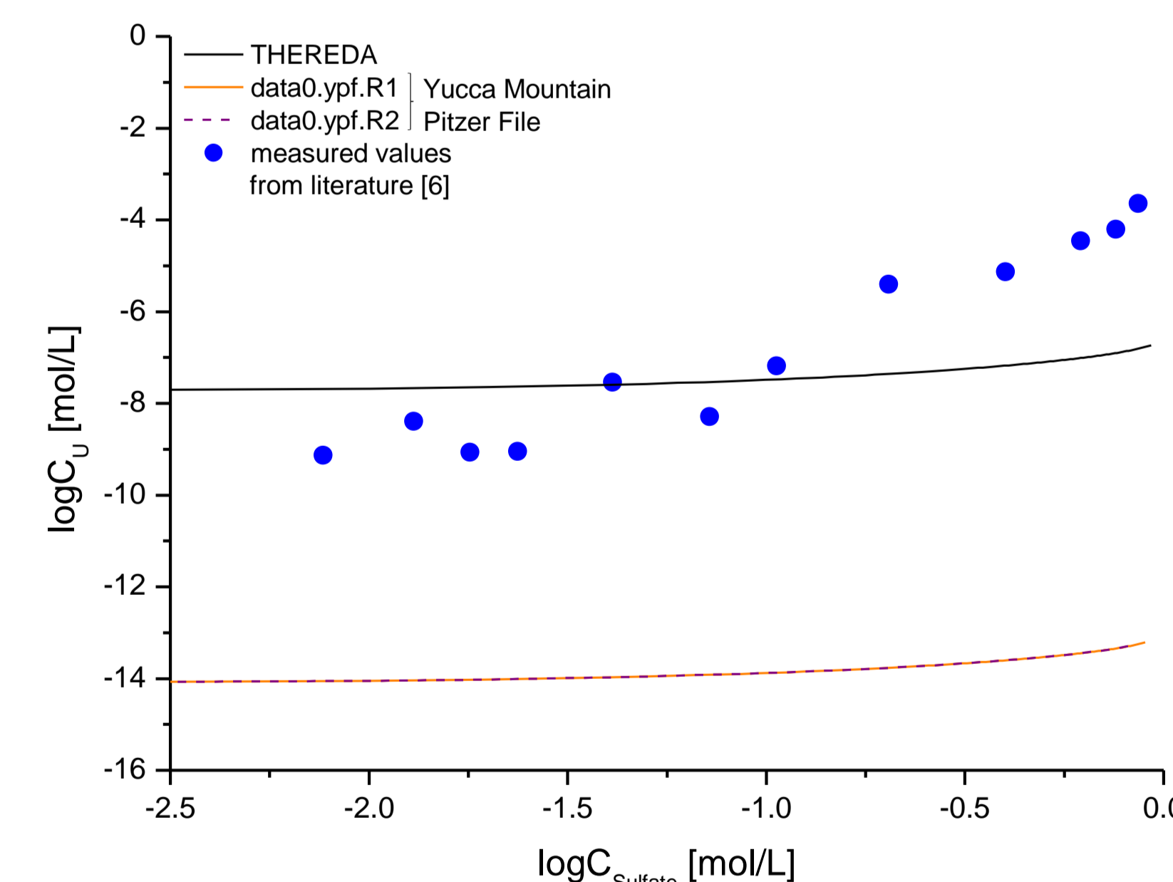
Fig. 3: Solubility of U(OH) 4 (am) in Na 2 SO 4 solution at T = 25 °C and log(C H+ ) = -4.5.
