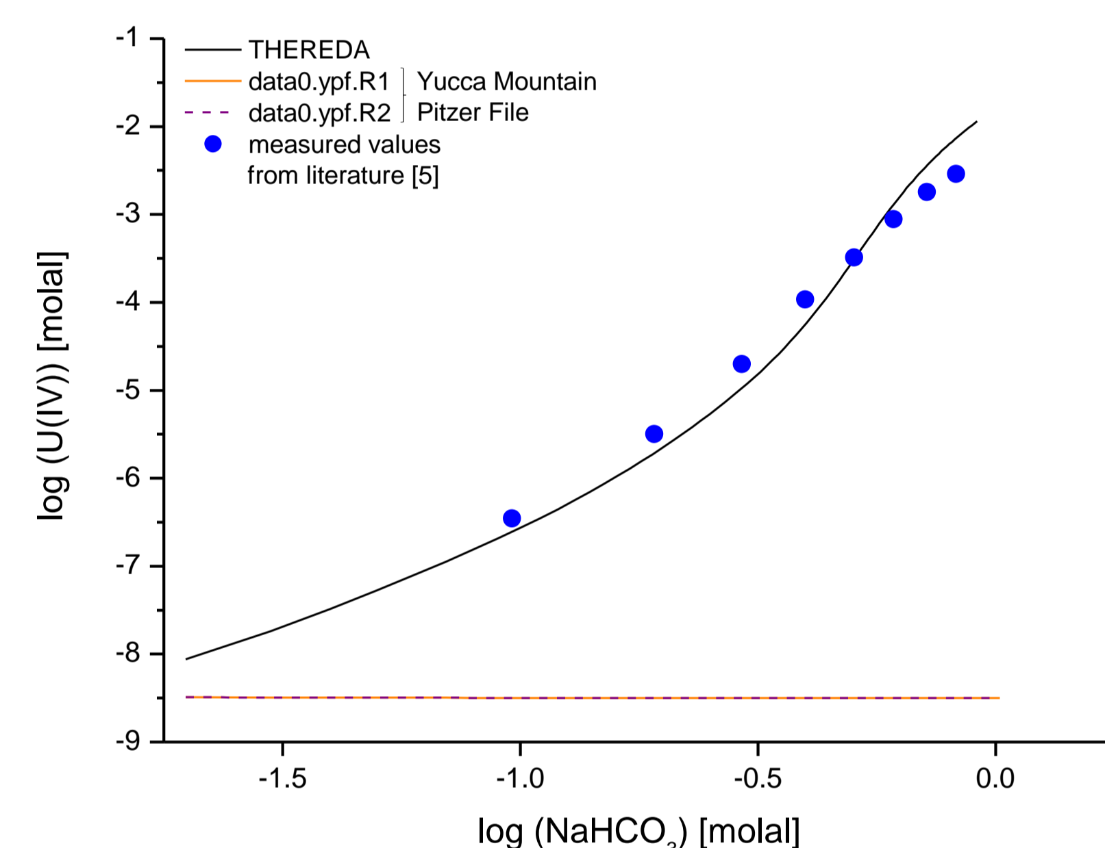
Fig. 2: Solubility of U(OH) 4 (am) in NaHCO 3 solution at T = 25 °C.
